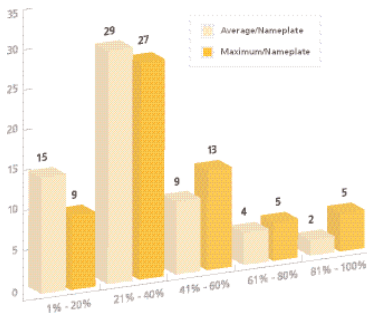
Variability in server power consumption relative to nameplate rating.
